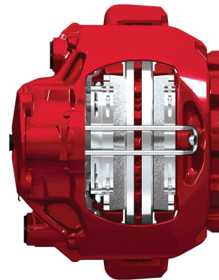
Pads and rotor are in compression making it a good application for semi-metallic friction material.
