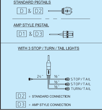
REAR SILL HARNESS STOP/TURN/TAIL LIGHT OPTIONS
