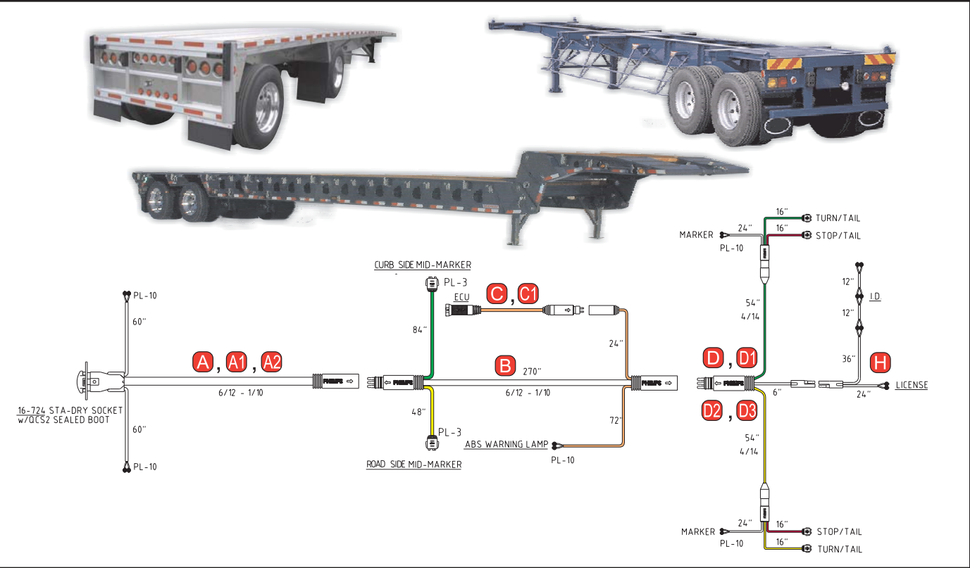
REAR SILL HARNESS STOP/TURN/TAI LIGHT OPTIONS
