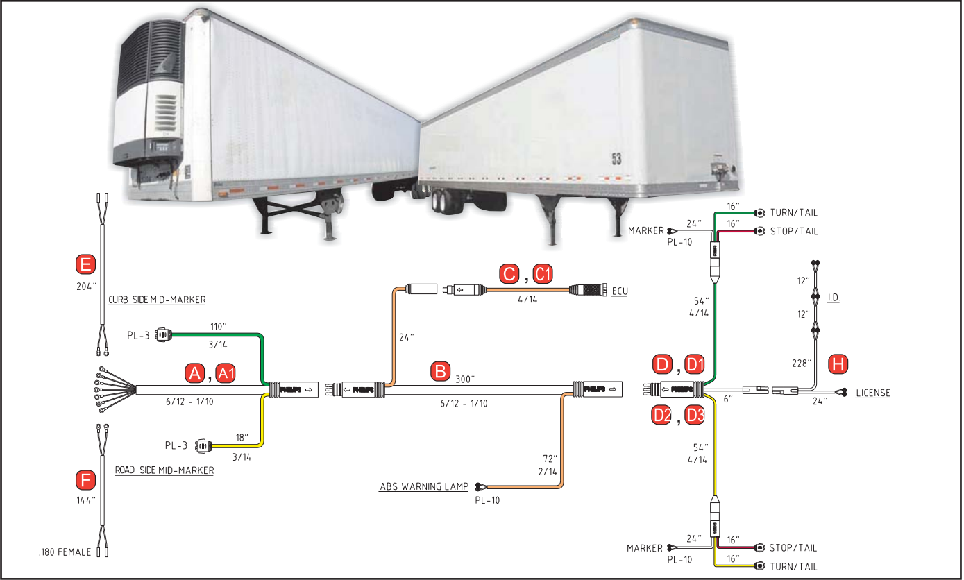
Standard (Length as shown above)
