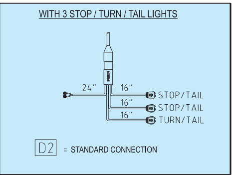
REAR SILL HARNESS STOP/TURN/TAI LIGHT OPTIONS
