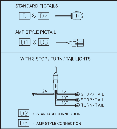
REAR SILL HARNESS STOP/TURN/TAI LIGHT OPTIONS
